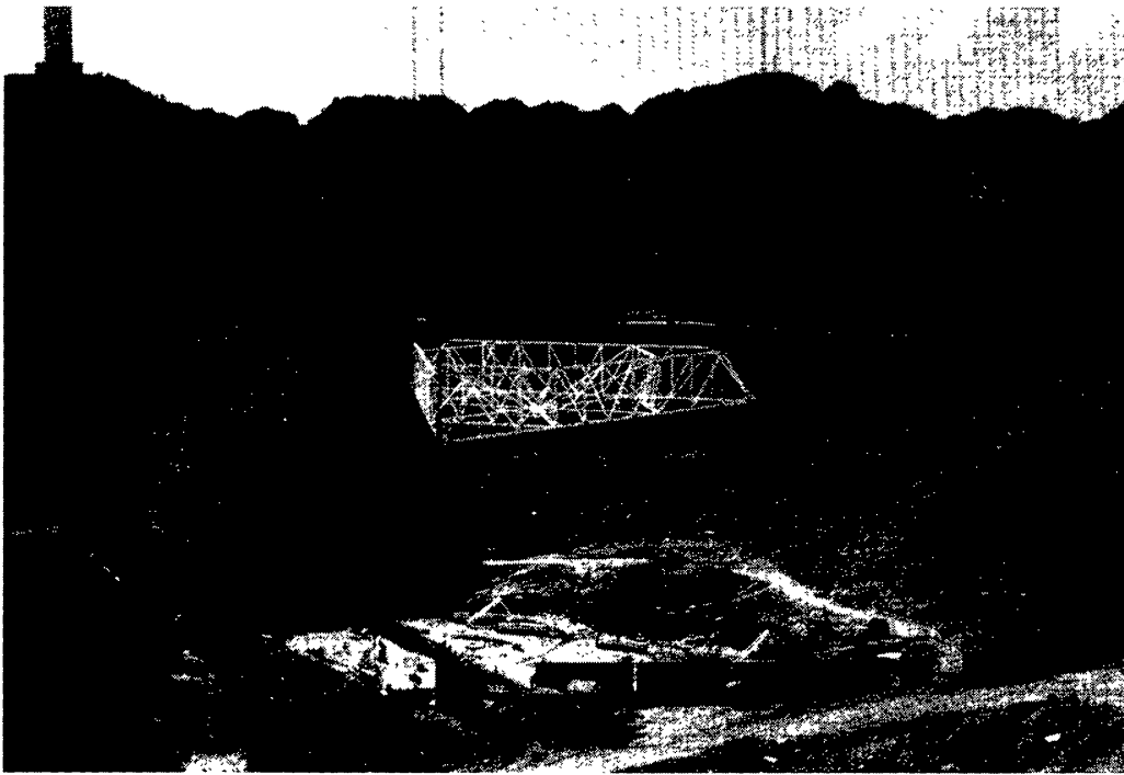
Figure 5. The triangular platform was raised with pulleys attached to auxiliary cables strung between the three towers.
