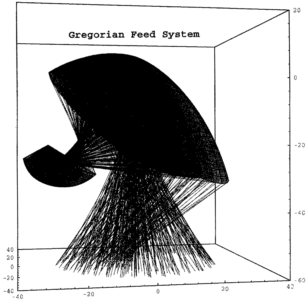
Figure 15. Two sub reflectors correct for the spherical aberration of the primary as shown. Compare with Figure 10(b).
