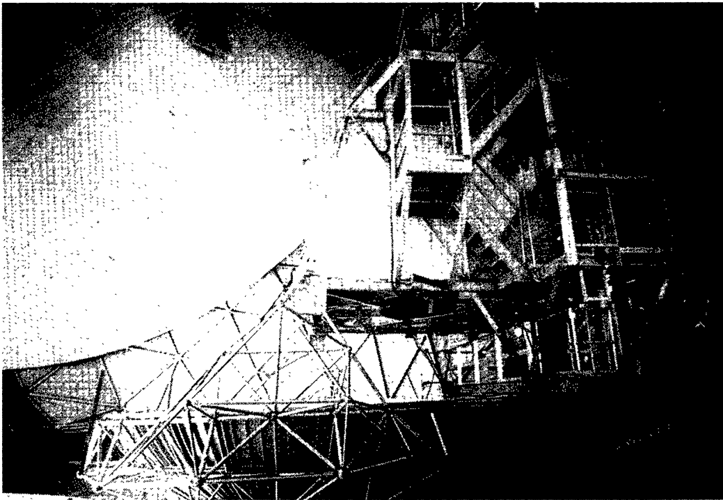
Figure 16. A view inside the Gregorian showing part of the secondary reflector, the tertiary (bottom) and the feed tower.
