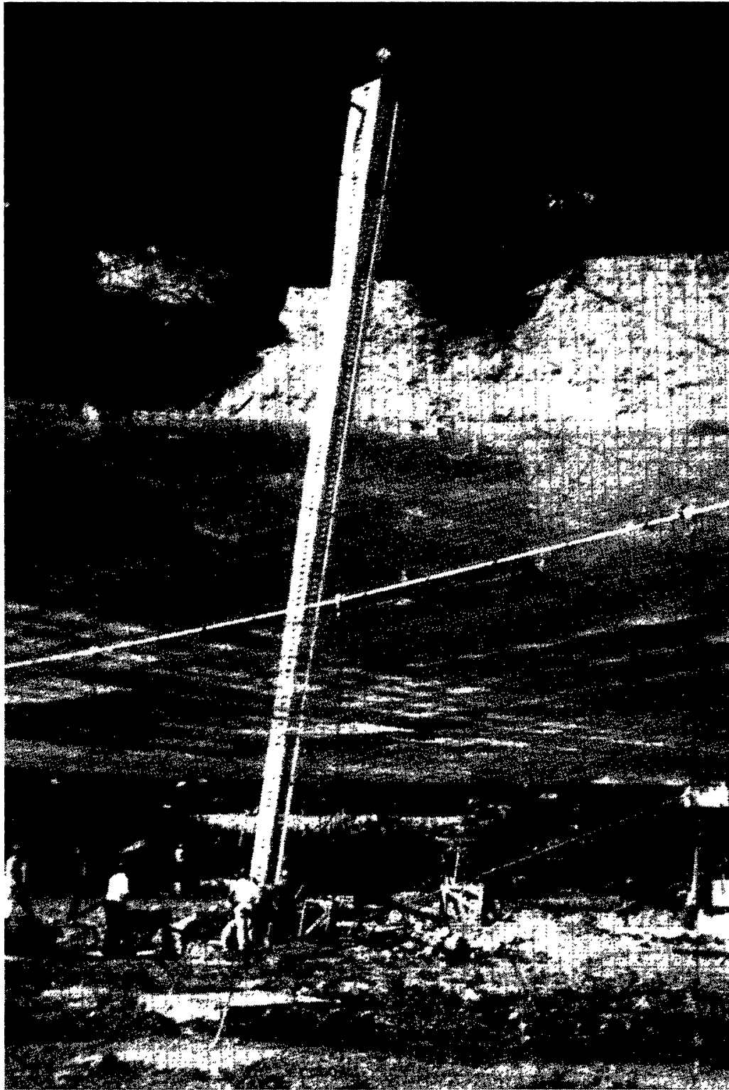
Figure 8. August 14, 1963, the 430-MHz line feed is lifted.
